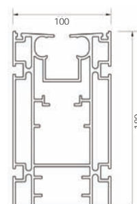
Maximum unsupported span 7200mm
